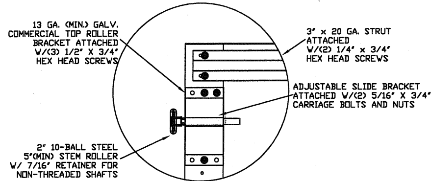
TYPICAL TOP FIXTURES N.T.S. ①
